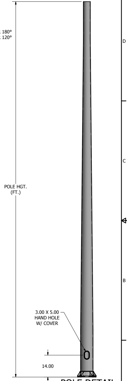
POLE DETAIL
